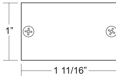
560-LED dimensions
